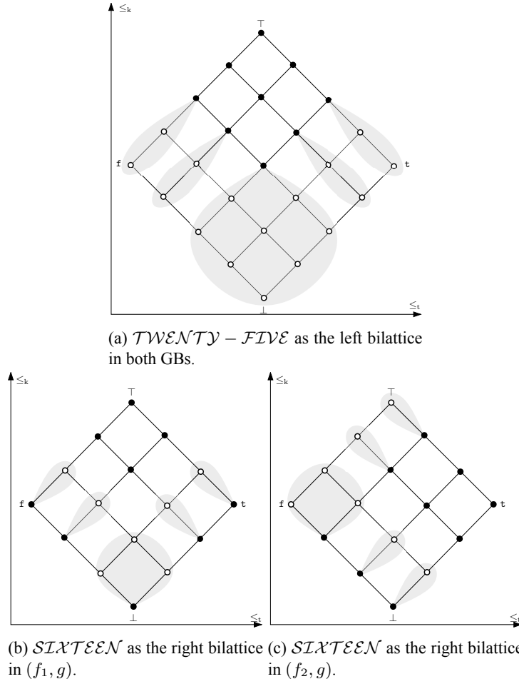
Figure 3.3: Representation of two regular k -directional GBs, (f_1, g) and (f_2, g) , demonstrating two of the ways that SIXTEEN can be seen as a common core between TWENTY-FIVE and SIXTEEN .
